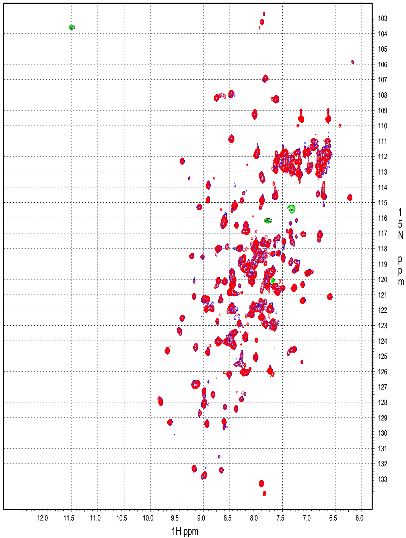
^{15}\text{N} Pixj Pfr (blue-pos./black-neg.) vs. Pfr 5 days later (red-pos./green-neg.) @ 600 MHz 25 C
